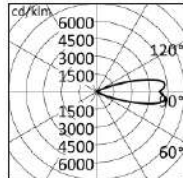
D44K/P01-LWWEB-AL
